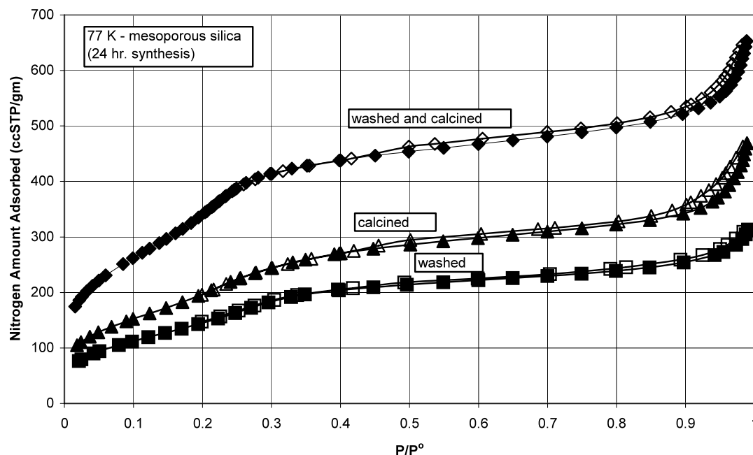
Fig. 3 Nitrogen adsorption-desorption isotherms at 77 K for 24 h synthesis time. Filled symbols denote desorption
